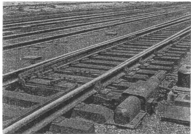
Electro-pneumatic switch movement with CP valve
